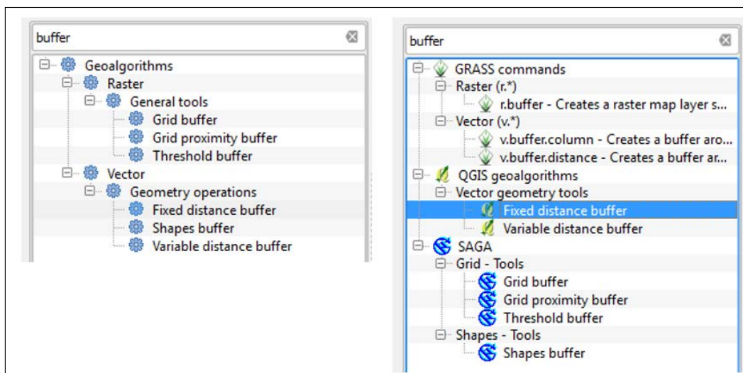
The Algorithms tab with buffer being used as the search term. The simplified interface is shown on the left and the advanced interface is on the right.
